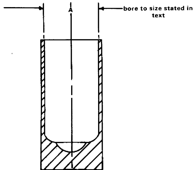
Fig. 44. Lightening cam followers.
