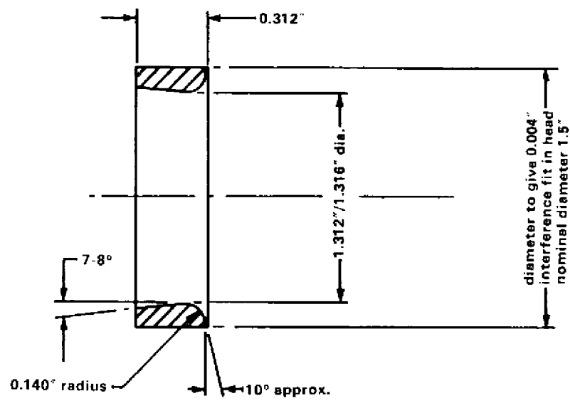
Fig. 33. Radiused valve seat insert.
