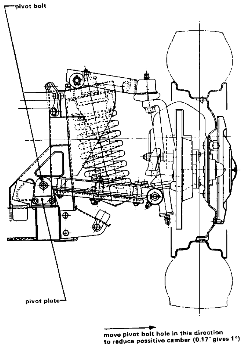
Fig. 54. Front suspension TR4.
