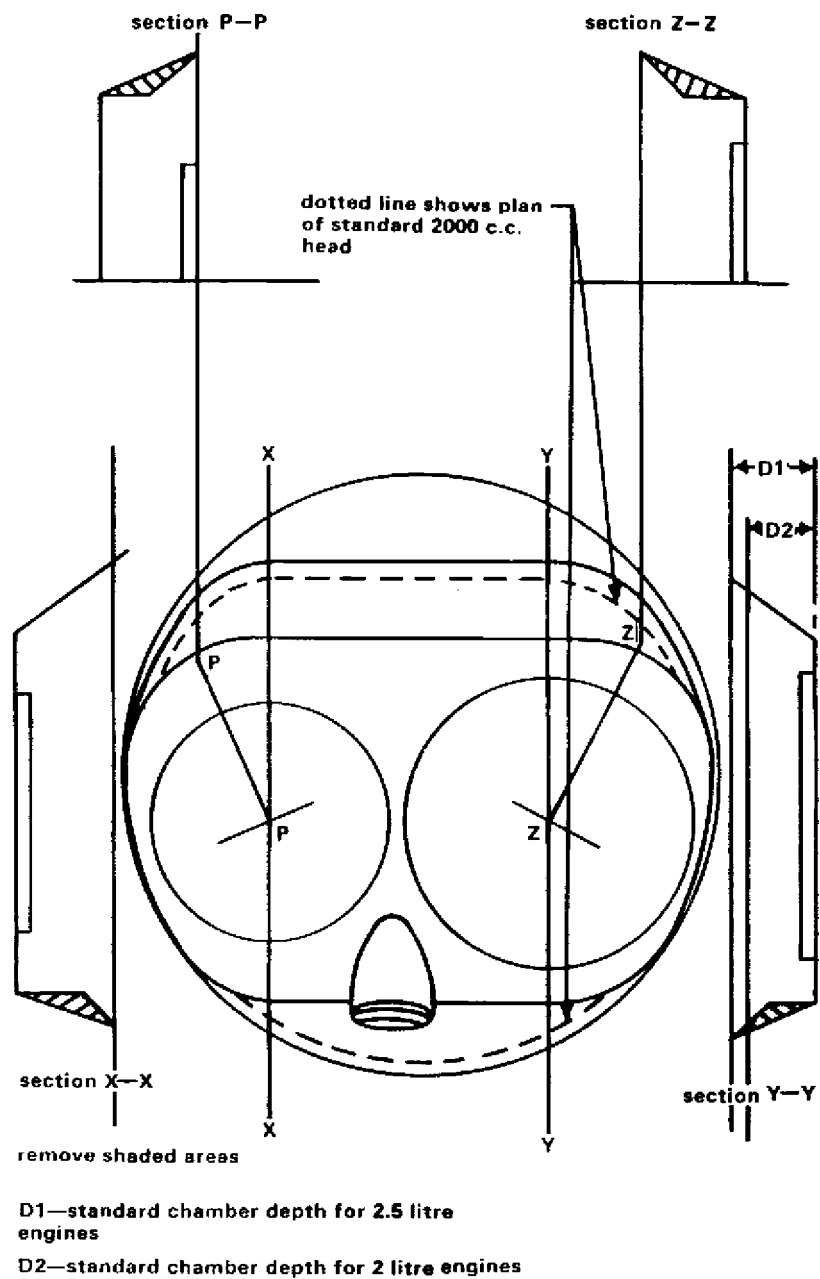
Fig. 28. Chamber modifications for TR5 and 6, 2500PI, Mk. 2 GT6, later type Triumph 2000 and Mk. 2 2000 Vitesse.
