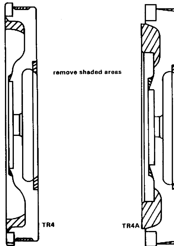
Fig. 46. Flywheel lightening.
