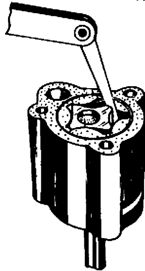
Fig. 6. Measuring clearance between outer rotor and body.
