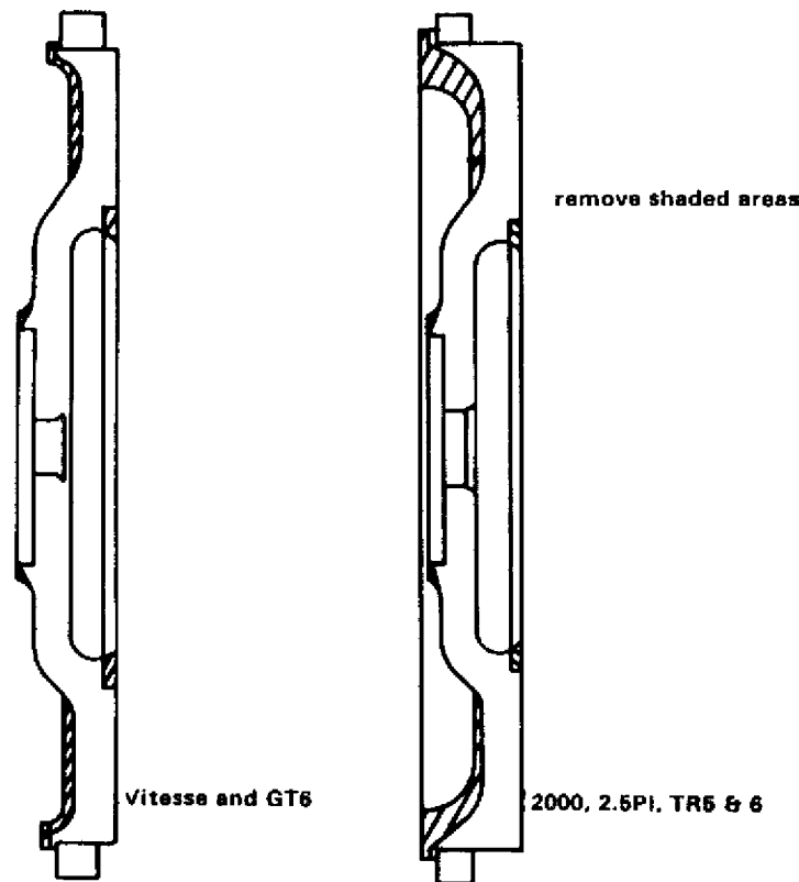
Fig. 46. Flywheel lightening.
