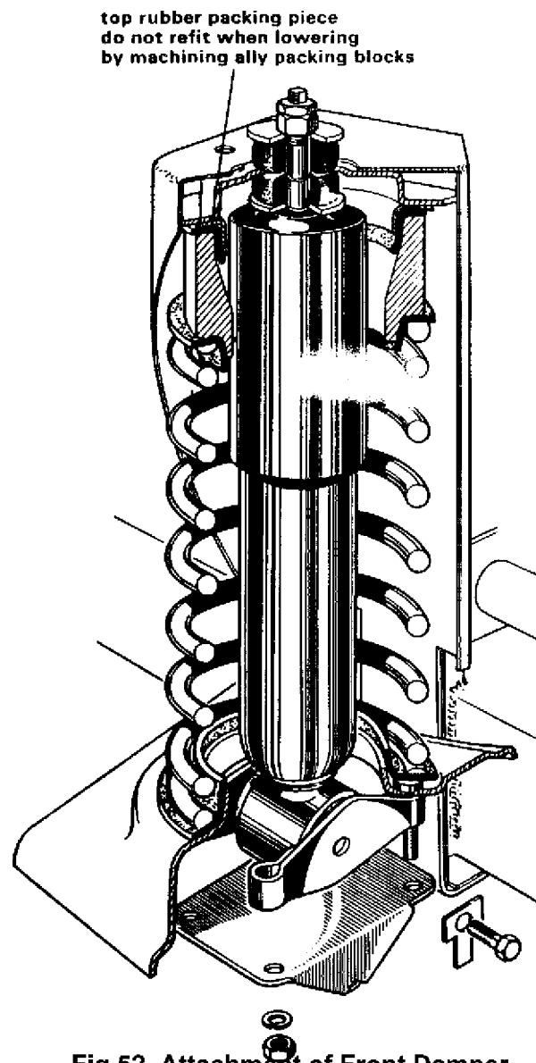
Fig 52. Attachment of Front Damper
