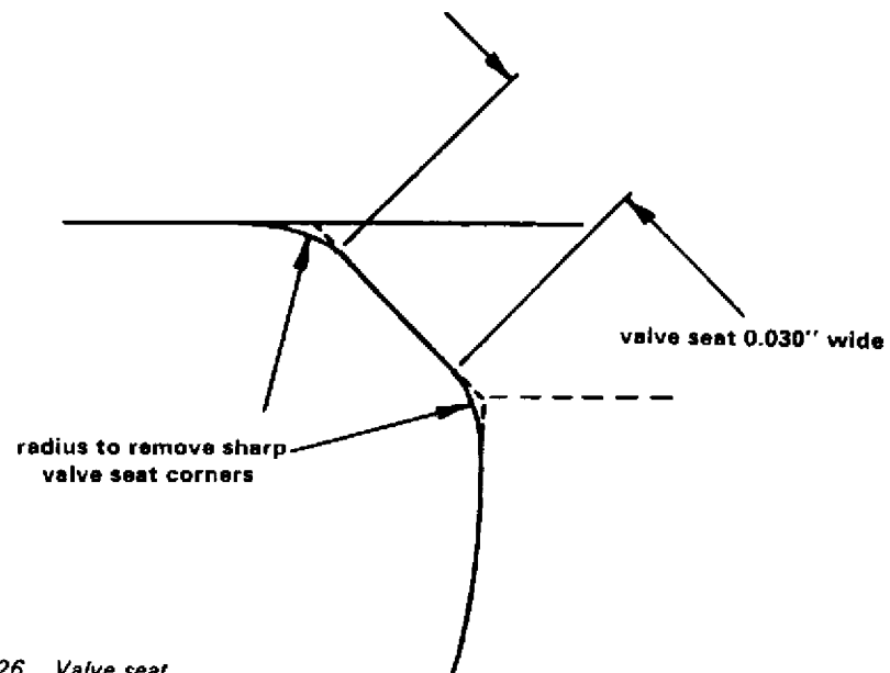
Fig. 26. Valve seat.
