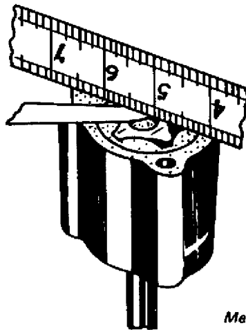
Fig. 6. Measuring clearance between outer rotor and body.
